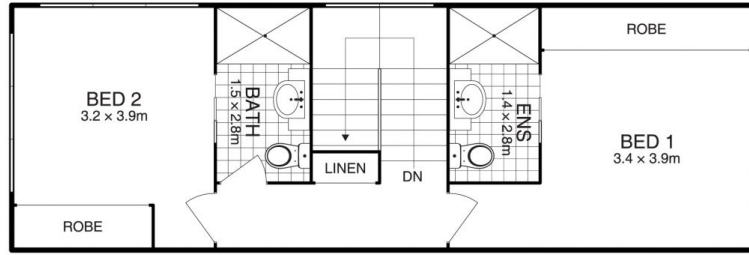
UPPER FLOOR
