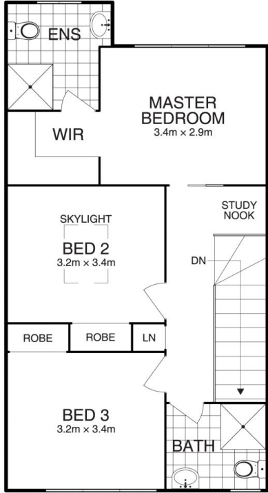
UPPER FLOOR
