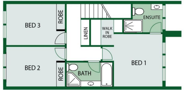
UPPER FLOOR
