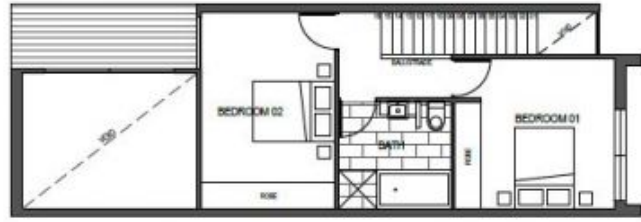
UPPER FLOOR PLAN
