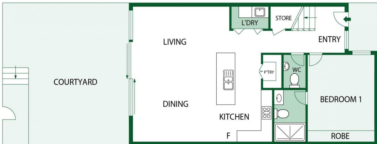
GROUND FLOOR
